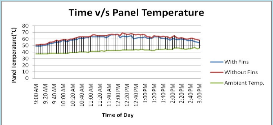
Fig. 16 - Comparison of PV panel temperatures with & without fin cooling.
