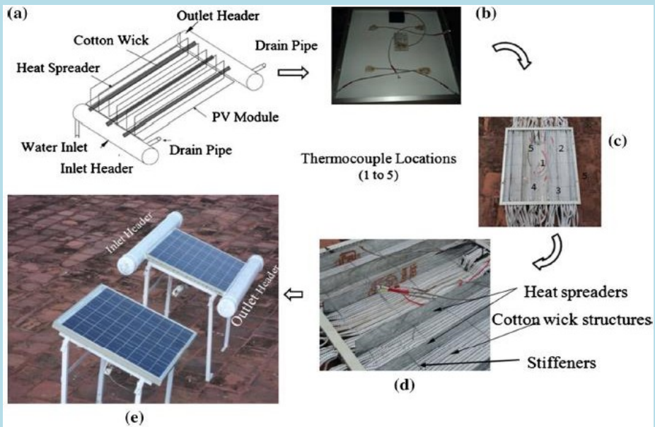
Fig. 15 - Photographic view of the experimental PV module with stages of fabrication. (a) Desired rear side of PV module (b) location of thermocouples (c) fins in conjunction with wick structures (d) details of the stiffeners and (e) final fabricated experimental setup with headers.
