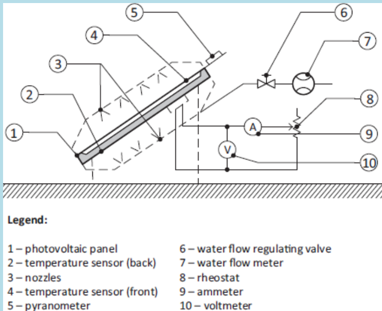
Fig. 8 - Schematic layout of the specific experimental setup
